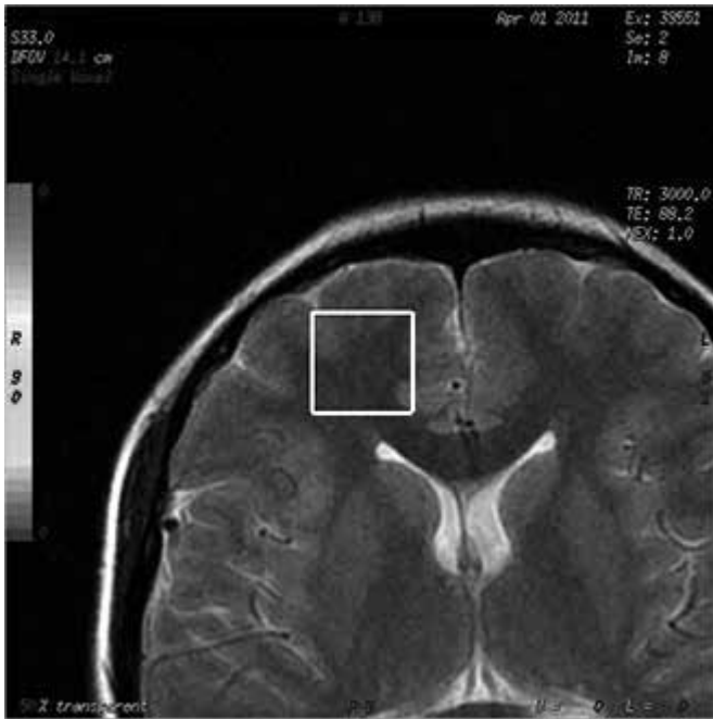
Figure 1. Proton magnetic resonance spectroscopy (1H-MRS) scan region in right prefrontal cortex of a patient with major depressive disorder-first episode.
